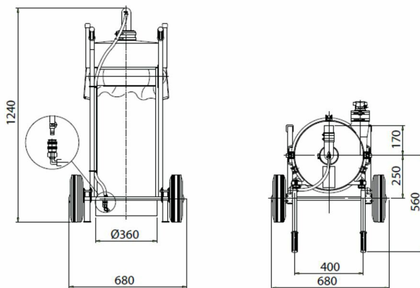
Dimensions FA7 70 liter.
